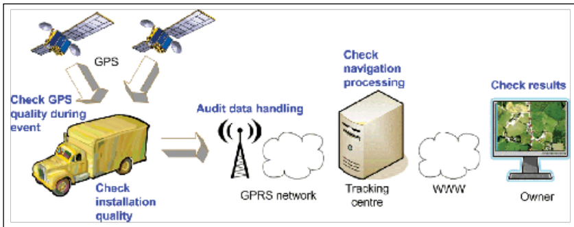
▲ FIGURE 2 Vehicle tracking system with checks (in blue) to establish quality of evidence
