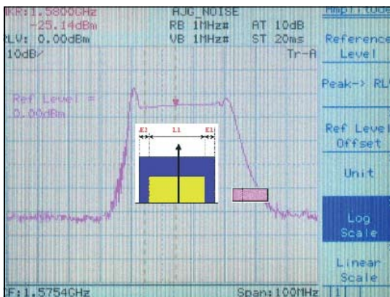
▲ FIGURE 3 Signal spectrum radiated by low-power jammer
